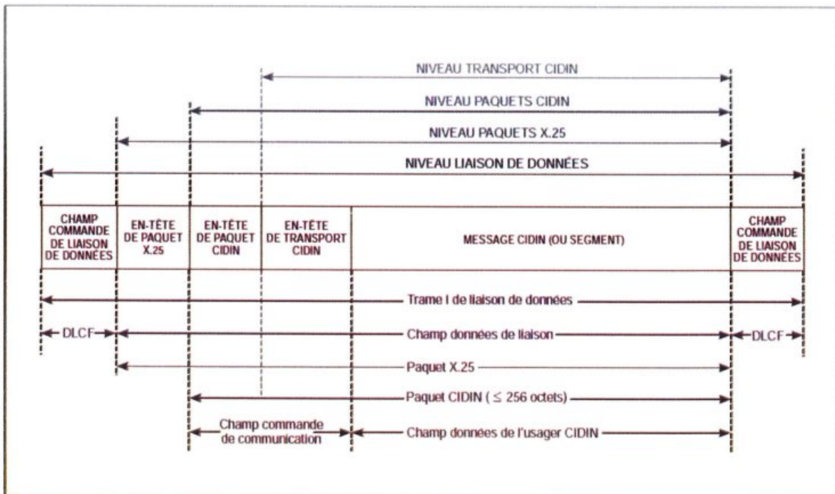
Figure 8-2. Terminologie CIDIN
